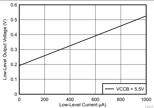
V_{CCA} = 3.0V V_{IL(A)} = 0.15V Figure 5-2. Low-Level Output Voltage ( V_{OL(Bx)} ) vs Low-Level Current ( I_{OL(Bx)} )
