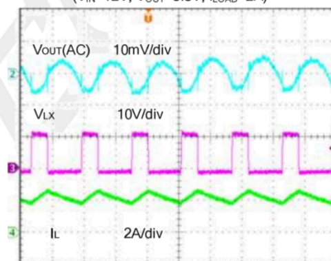
Output Ripple
