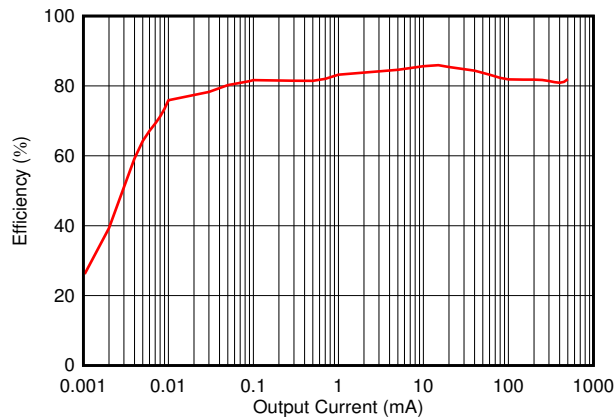
图 8-5. TPS7A11 Output Efficiency at 1.2 V IN and 1.0 V OUT
