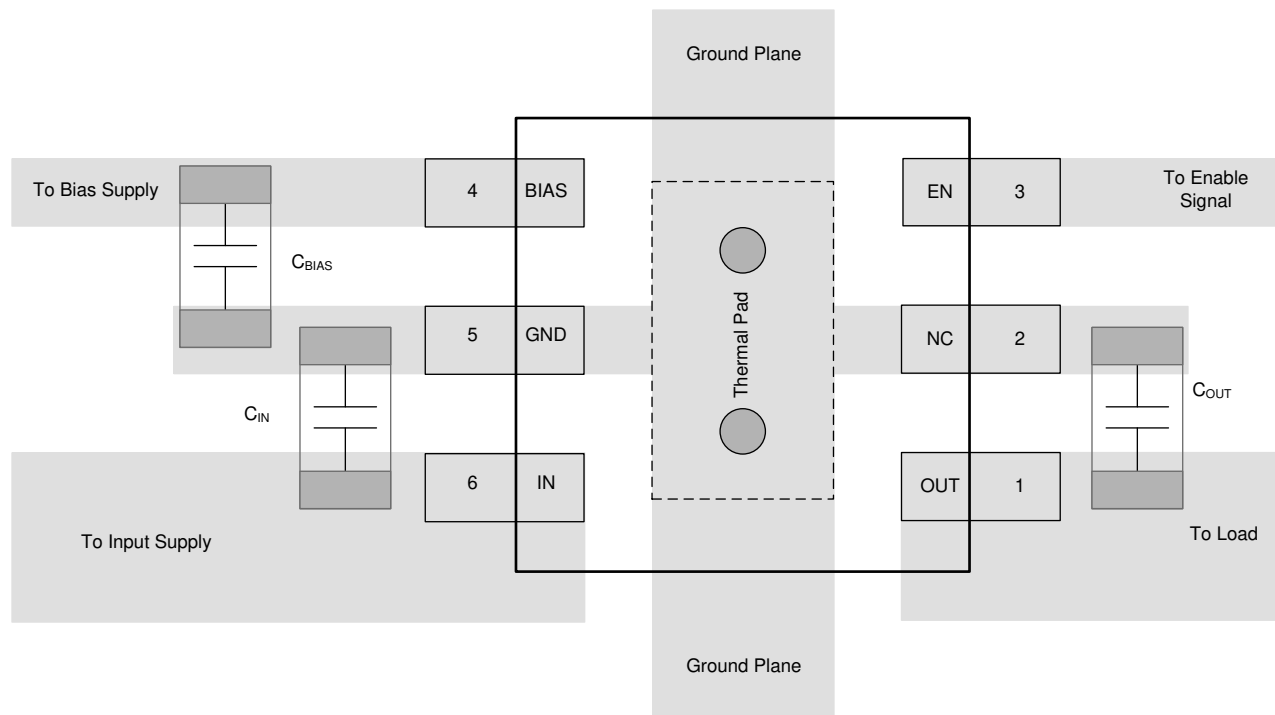
图 10-2. Recommended Layout for DRV Package
