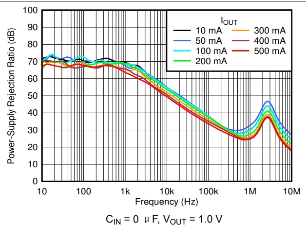
图 6-24. V_{IN} PSRR vs Frequency and I_{OUT}
