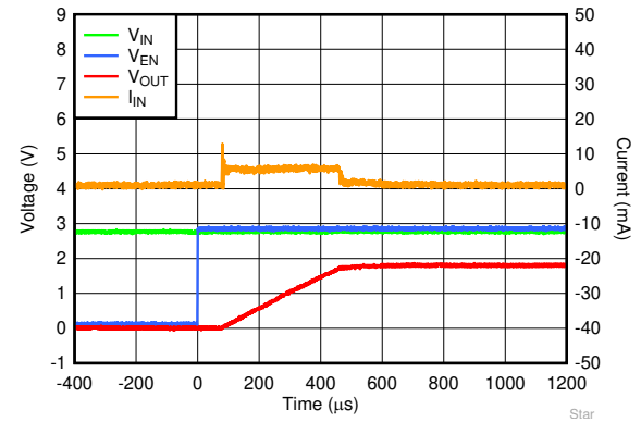
图 5-56. C_{OUT} = 1\mu\text{F} 时的启动浪涌电流
