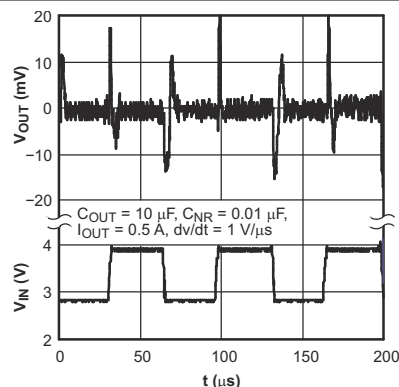
V_{OUT} = 1.8V (旧芯片)
