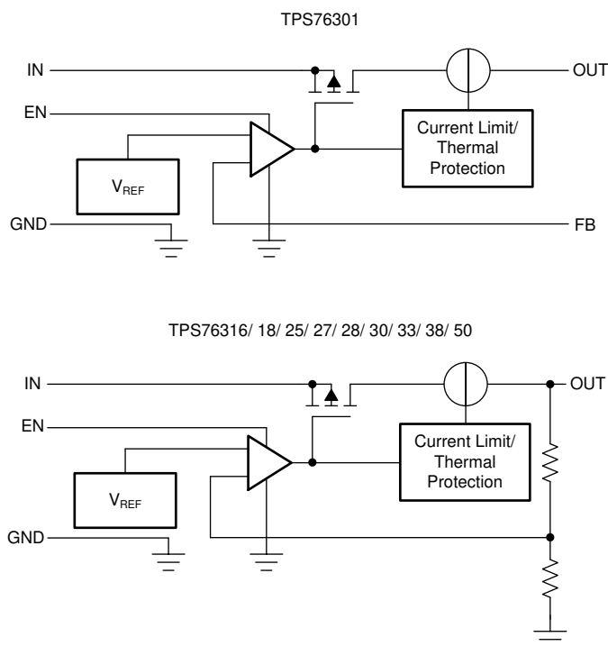
Figure 6-1. Functional Block Diagram (Legacy Chip)
