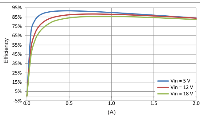
图 6-7. Efficiency, Forced PWM
