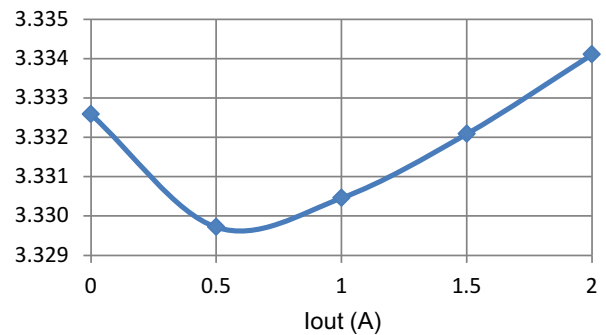
图 6-16. Load Regulation, 25^\circ\text{C} , 1% 100-PPM Resistor
