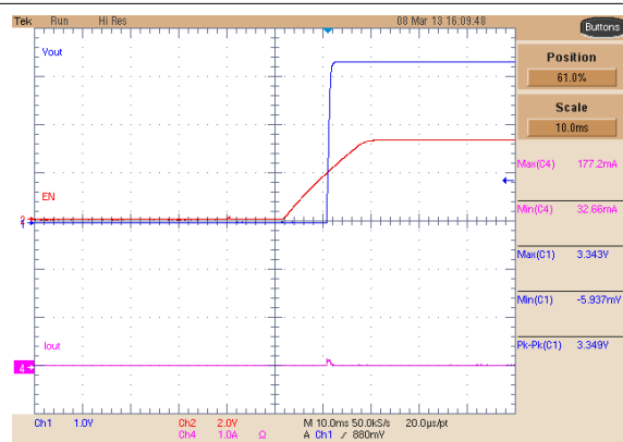
图 8-37. Buck 3 Start-Up
