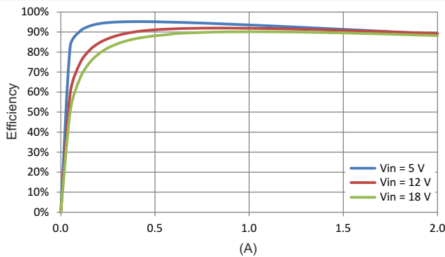
图 6-13. Efficiency, Forced PWM
