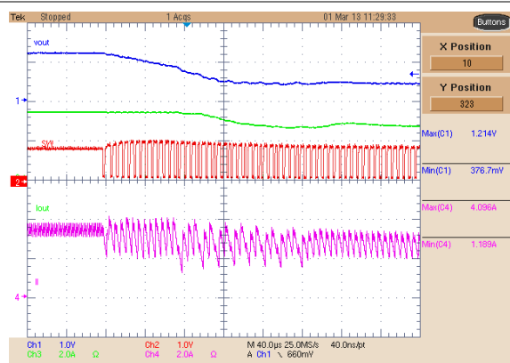
图 8-17. Buck 1 Current Limit Operation With Slow Rising Output Current, Trip at 4 A
