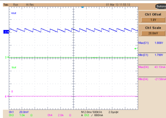
图 8-33. Buck 2 Low-Power Output, No Load
