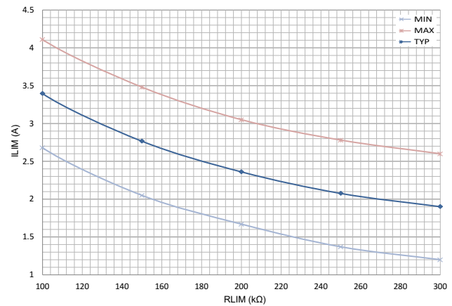
图 6-18. Current Limit V_{IN} = 12\text{ V} , f_{SW} = 500\text{ KHz}
