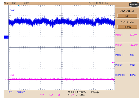
图 8-30. Buck 2 Ripple, No Load
