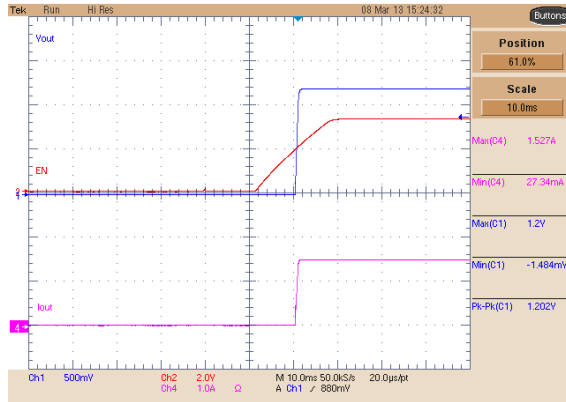
图 8-5. Buck 1 Start-Up 1.5-A Resistive
