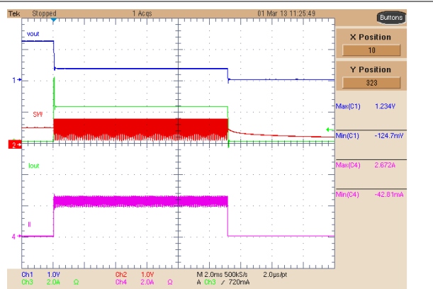
图 8-18. Buck 1 Current Limit Operation, Hiccup
