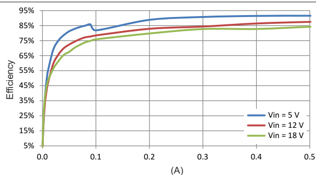
图 6-7. Efficiency, Forced PWM
