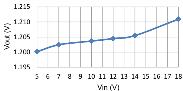
图 6-5. Line Regulation, Load = 1 A
