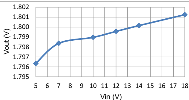
图 6-11. Line Regulation, Load = 1 A
