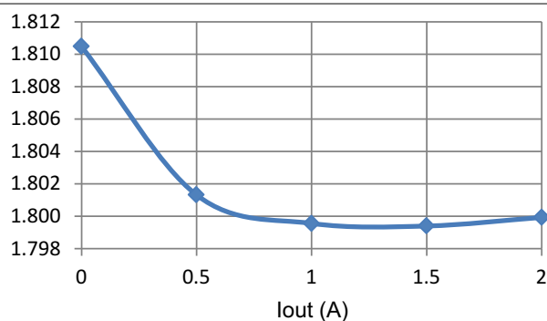
图 6-10. Load Regulation, 25^\circ\text{C} , 1% 100-PPM Resistor
