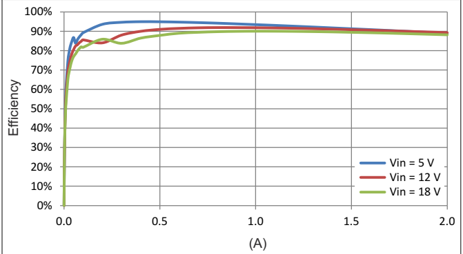
图 6-14. Efficiency, LOW_P Mode
