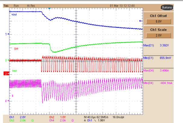
图 8-48. Buck 3 PFM to PWM Transition
