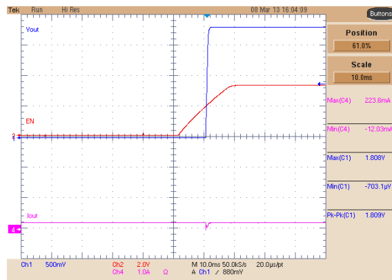
图 8-23. Buck 2 Start-Up, No Load
