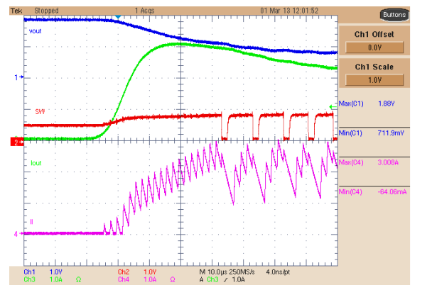
图 8-36. Buck 2 Current Limit Operation
