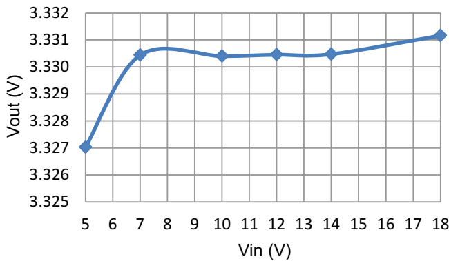
图 6-17. Line Regulation, Load = 1 A
