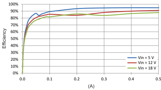
图 6-13. Efficiency, Forced PWM
