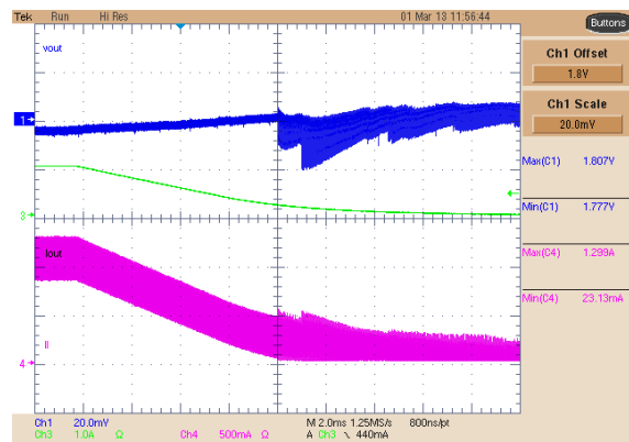
图 8-35. Buck 2 PWM to PFM Transition
