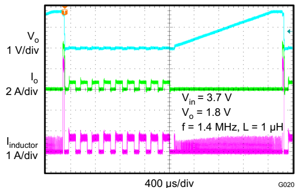
Figure 24. Hiccup Short Circuit Protection
