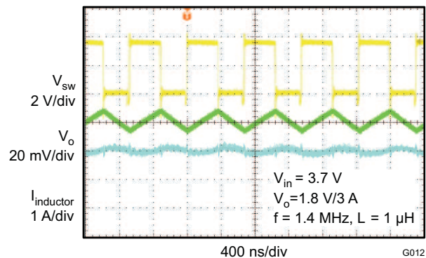
Figure 16. PWM Operation
