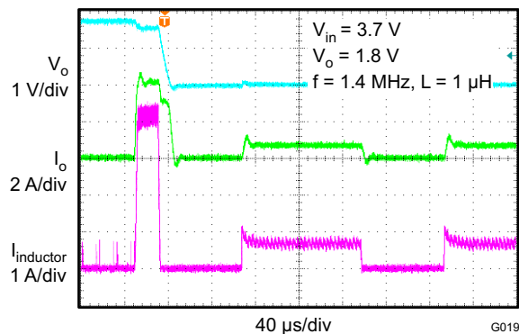
Figure 23. Hiccup Short Circuit Protection
