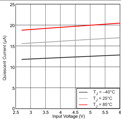
图 7-2. Quiescent Current vs Input Voltage
