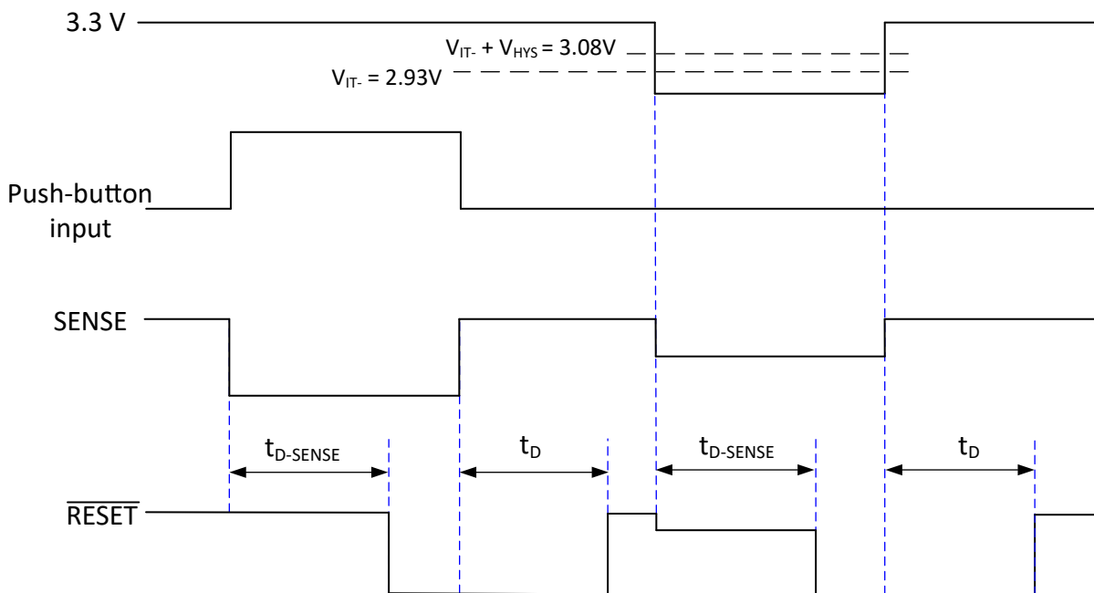
图 7-2. Design 1 Timing Diagram
