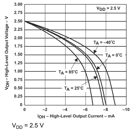
图 7-5. High-Level Output Voltage vs High-Level Output Current
