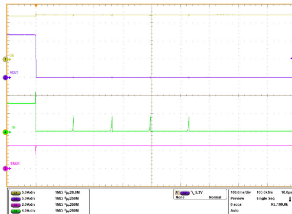
A. R_{LIM} = \text{TBD}\ \Omega C_{ITIMER} = 4.7\text{nF} C_{RETRY\_DLY} = 2.2\text{nF} , C_{NRETRY} = 2.2\text{nF}
