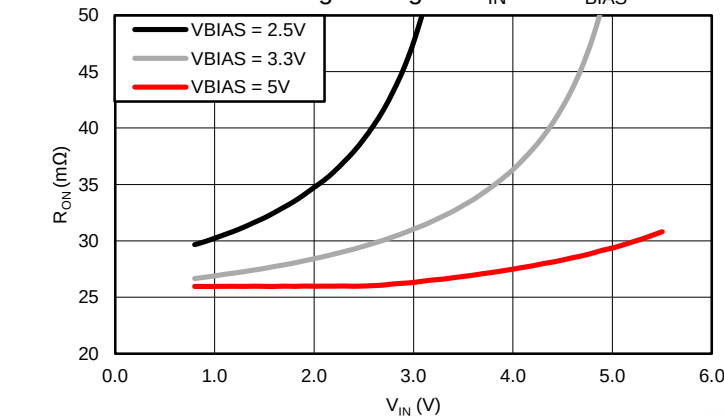
Figure 34. RON vs VIN
