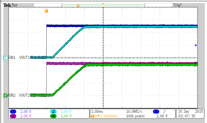
Figure 26. Turn-On Response Time ( V_{IN} = 0.8\ \text{V} , V_{BIAS} = 5\ \text{V} )
