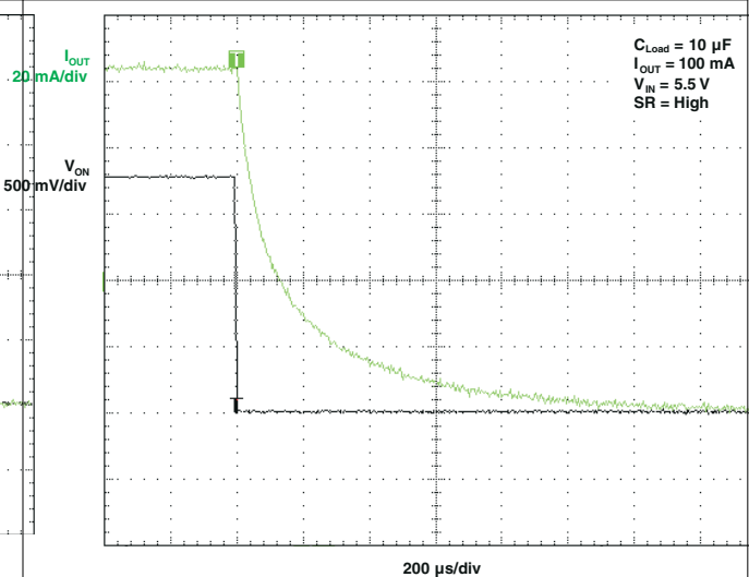
图 5-19. t_{OFF} Response
