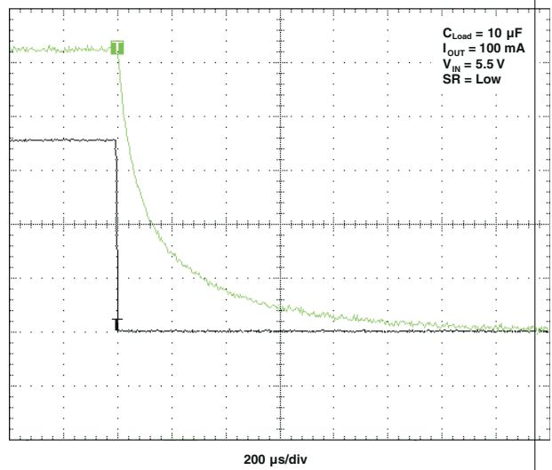
图 5-27. t_{OFF} Response
