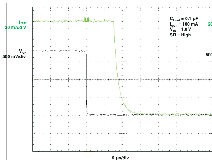
图 5-16. t_{OFF} Response
