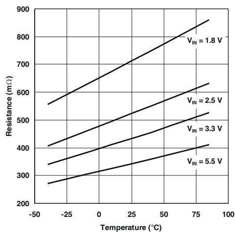
图 5-2. ON Resistance vs Temperature
