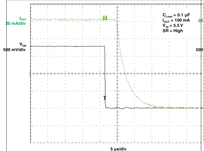
图 5-18. t_{OFF} Response
