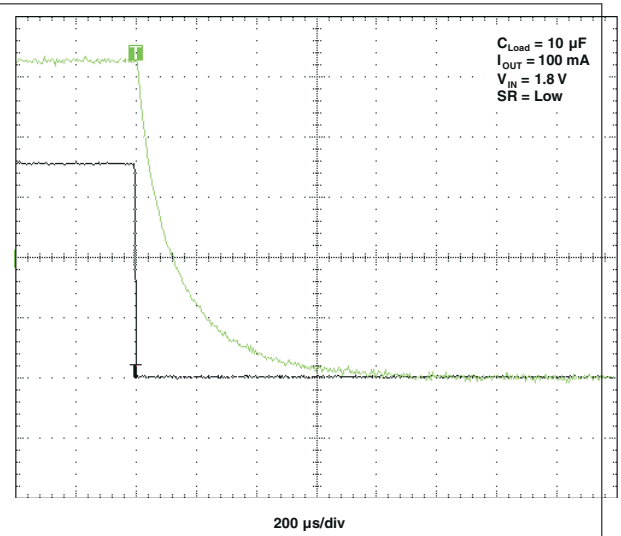
图 5-25. t_{OFF} Response
