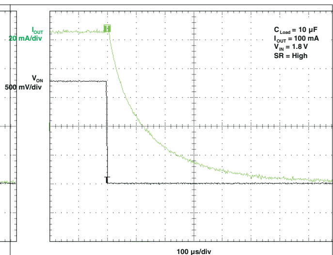
图 5-17. t_{OFF} Response
