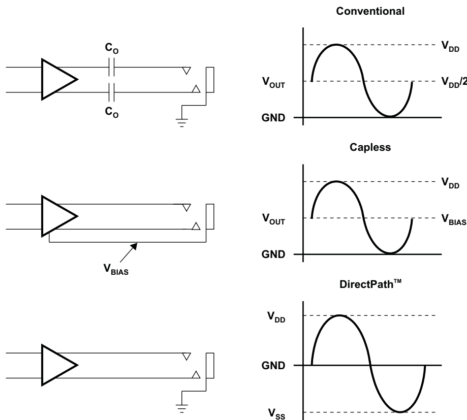
Figure 19. Amplifier Applications
