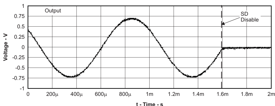
Figure 22. Shutdown Time
