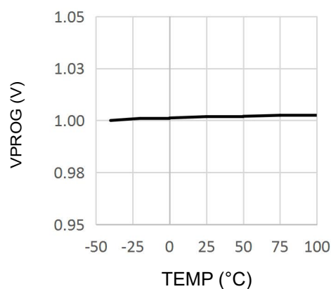
Figure 2: PROG Pin Voltage VS. Temperature Relationship Curve
