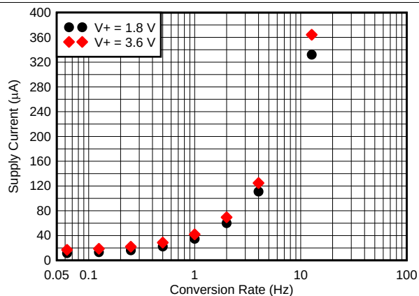
图 10. Quiescent Current vs Conversion Rate °
