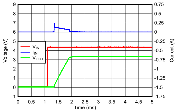
图 7-8. Inrush Current With 22\text{ }\mu\text{F} at C_{OUT}
