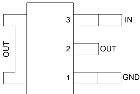
图 4-2. KVU Package, 3-Pin TO-252 (Top View)
