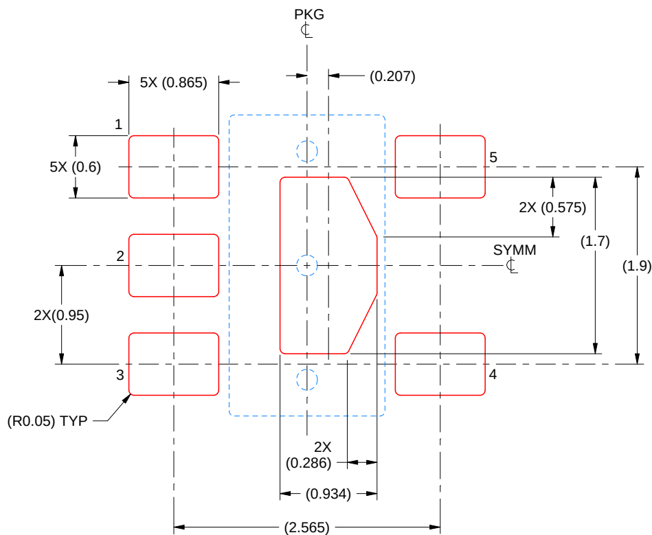
SOLDER PASTE EXAMPLE BASED ON 0.125 mm THICK STENCIL SCALE:20X
