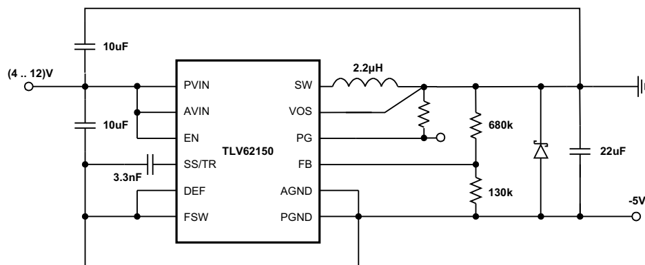
Figure 38. -5-V Inverting Power Supply
