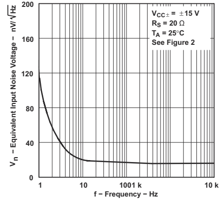
Figure 6-44. Equivalent Input Noise Voltage vs Frequency
