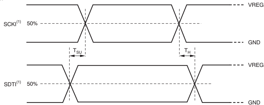
Figure 1. Input Timing
