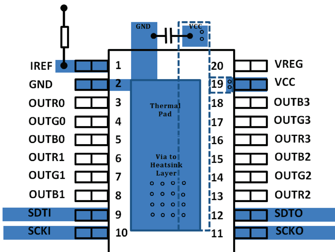
Figure 40. Layout Example
