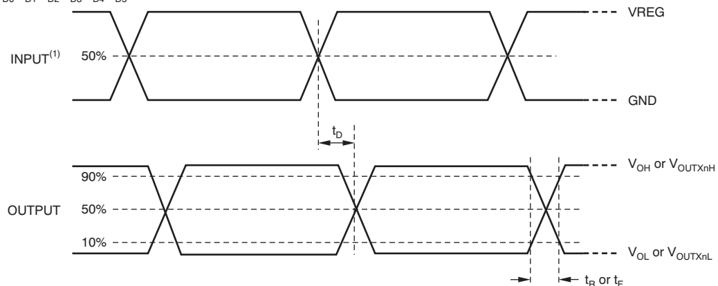
Figure 2. Output Timing
