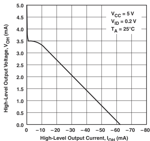
Figure 5-3. High-Level Output Voltage vs High-Level Output Current
