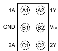
Figure 5-4. YFP Package 6-Pin DSBGA Transparent Top View
