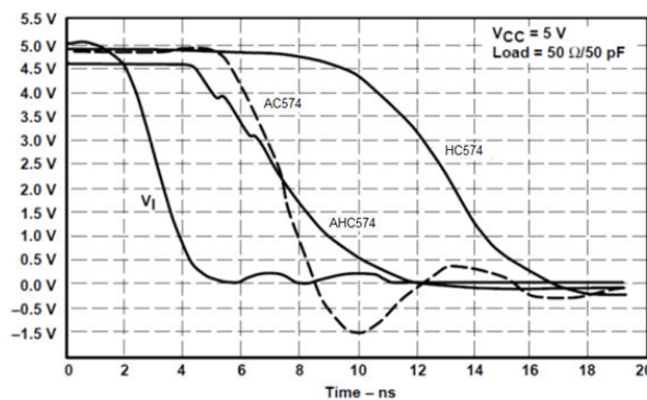
图 8-2. Switching Charactersitics Comparison
