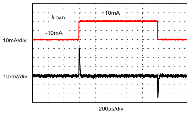
C_L = 1\ \mu\text{F} , I_{\text{OUT}} = 10\text{mA}
