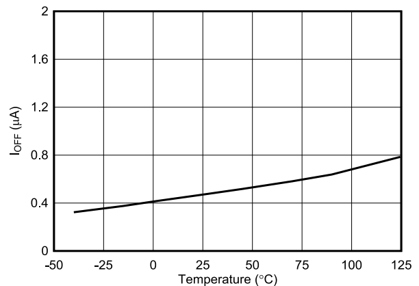
Figure 6-42. Shutdown Current vs Temperature
