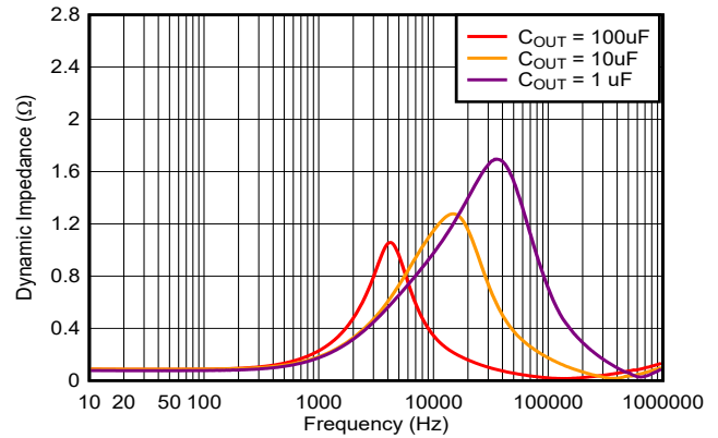
Figure 6-40. Output Impedance
