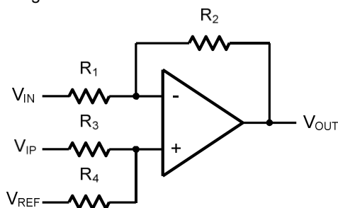
Figure 4. Differential Amplifier
