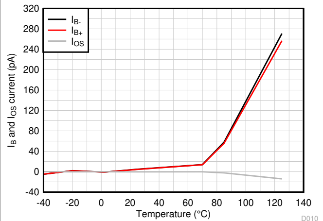
图 7-48. I_B and I_{OS} vs Temperature
