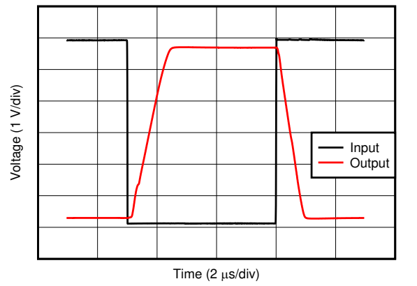
图 7-30. Overload Recovery
