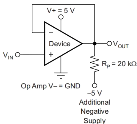
Figure 19. V_{OUT} 接地范围
