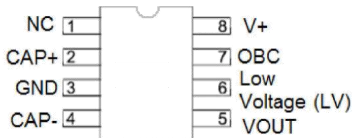
DIP-8/SOP-8/MSOP-8
