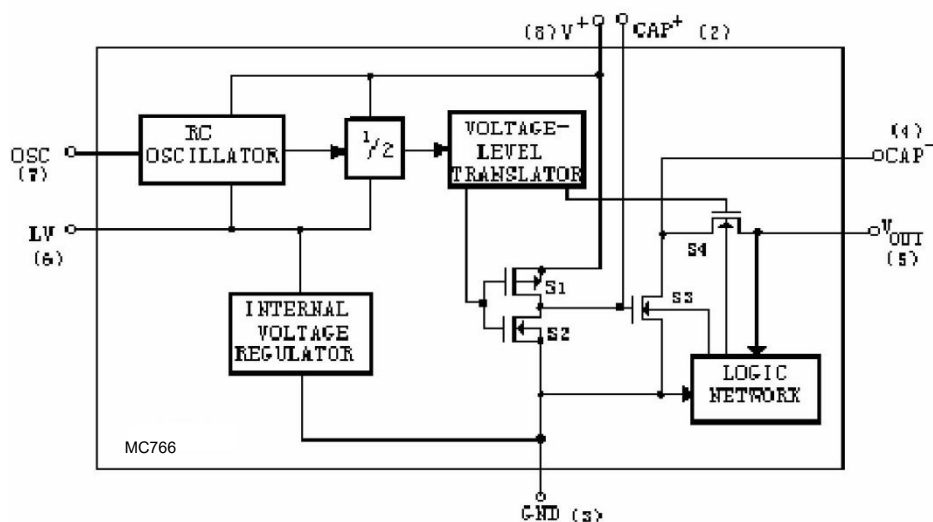
Block of function module in chip
