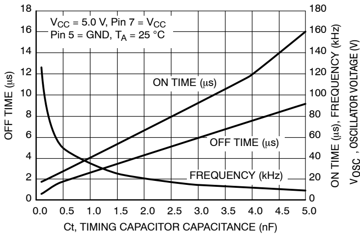
Figure 3. Oscillator Frequency
