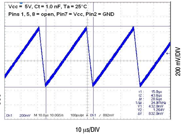
Figure 4. Timing Capacitor Waveform
