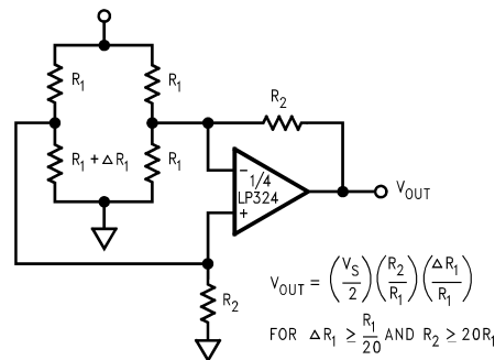
Figure 24. Bridge Current Amplifier
