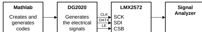
图 182. Application Example Test Setup
