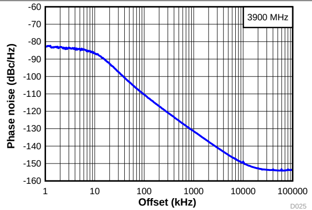
图 12. Narrow Band Phase Noise at 3.9 GHz
