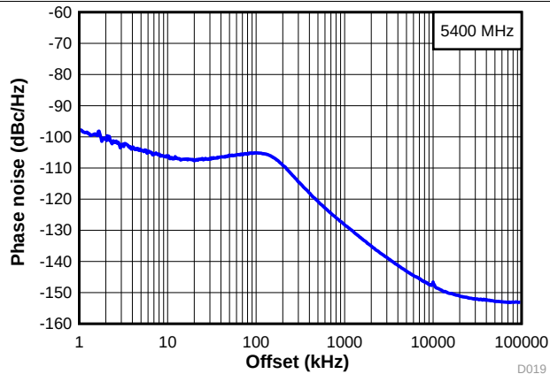
图 17. Wide Band Phase Noise at 5.4 GHz
