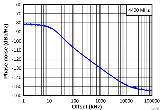
图 14. Narrow Band Phase Noise at 4.4 GHz
