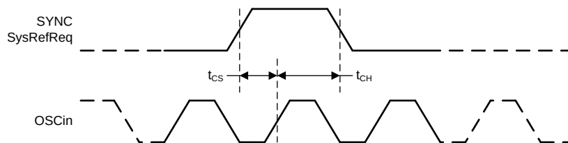
图 2. Trigger Signals Timing Diagram
