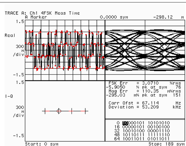
图 184. Gaussian 4FSK Modulation Quality
