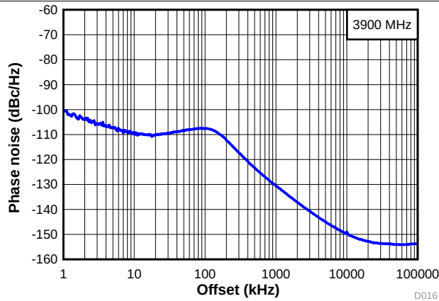
图 11. Wide Band Phase Noise at 3.9 GHz
