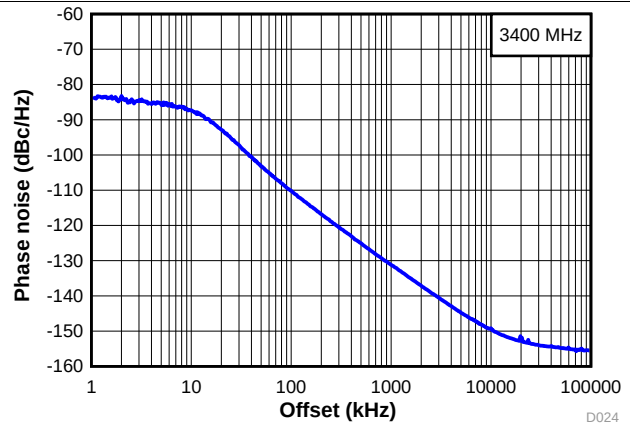
图 10. Narrow Band Phase Noise at 3.4 GHz
