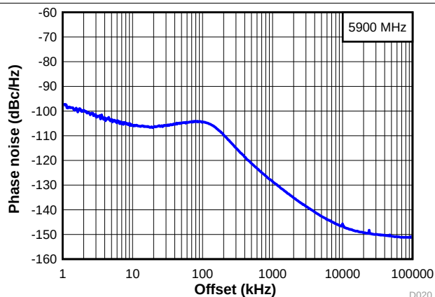
图 19. Wide Band Phase Noise at 5.9 GHz
