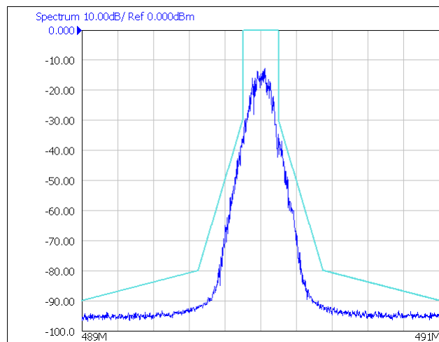
图 171. Gaussian 4FSK Modulated Spectrum
