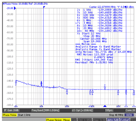
Figure 27. OSCout, 122.88 MHz, LVCMOS (Norm/Inv) Normal Output Measured, Inverse 50-Ω Termination
