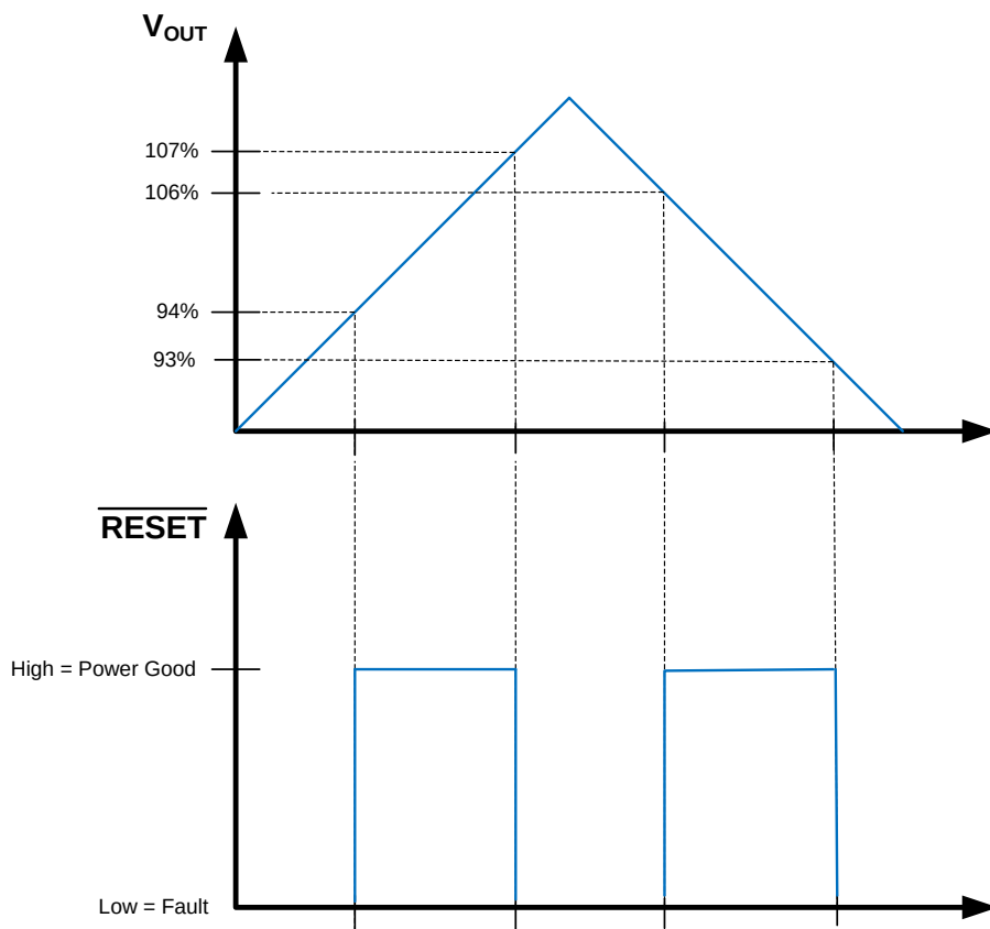
Figure 7. Static RESET Operation
