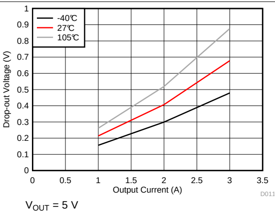
Figure 23. Drop-out for -1% Regulation
