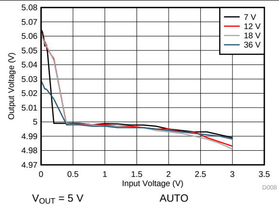
Figure 20. Load and Line Regulation
