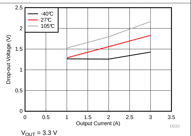
Figure 36. Drop-out for \geq 1.85\text{ MHz}
