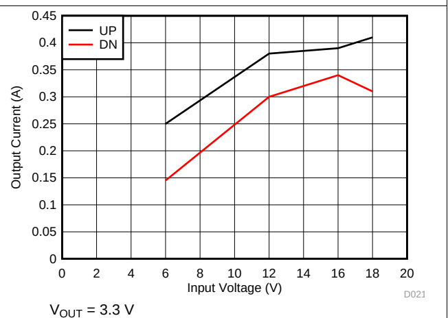
Figure 34. Load Current for Mode Change
