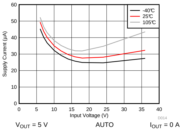
Figure 21. Input Supply Current
