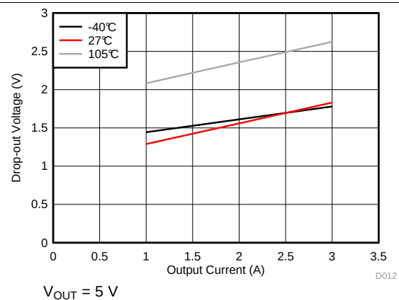
Figure 24. Drop-out for \geq 1.85\text{ MHz}
