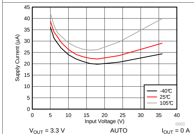
Figure 33. Input Supply Current
