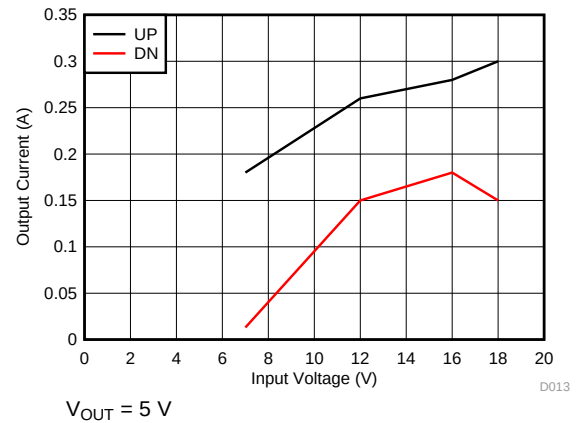
Figure 22. Load Current for Mode Change
