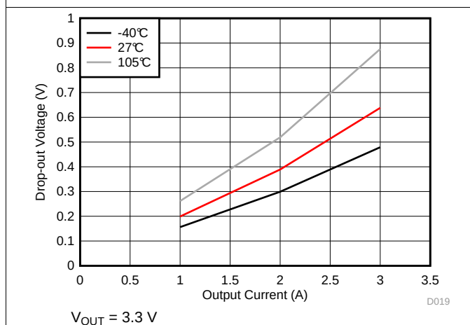
Figure 35. Drop-out for -1% Regulation
