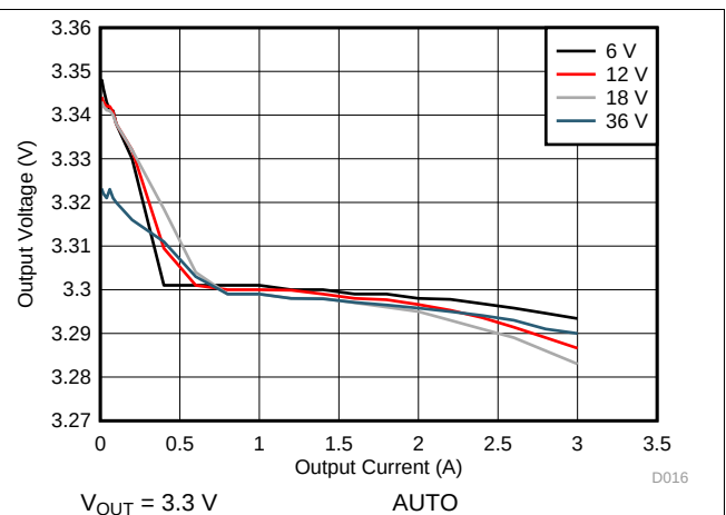
Figure 32. Load and Line Regulation
