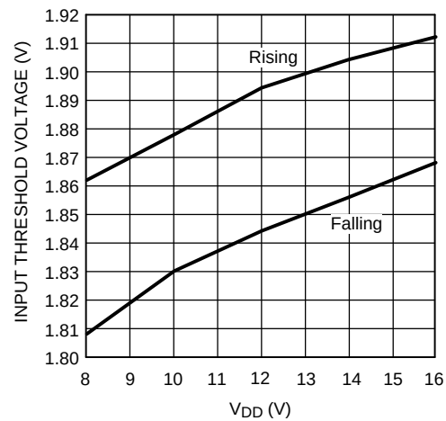
Figure 13. Input Thresholds vs Supply Voltage
