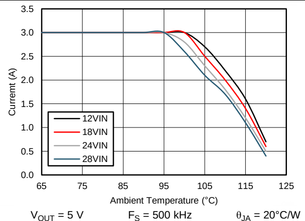
Figure 78. Derating Curve
