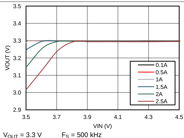
Figure 13. Dropout Curve
