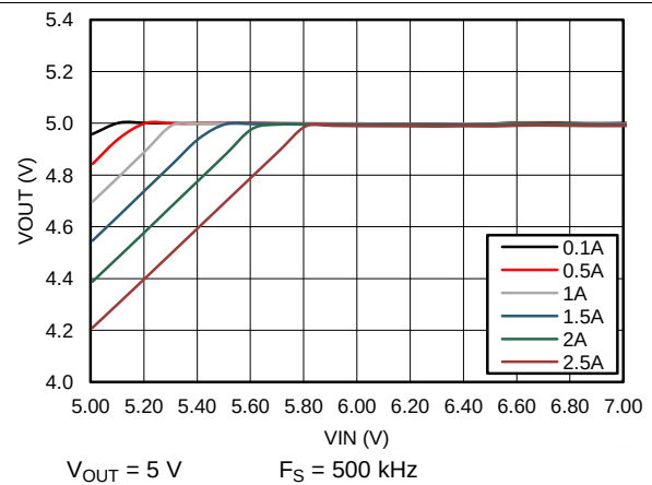
Figure 76. Drop-out Curve
