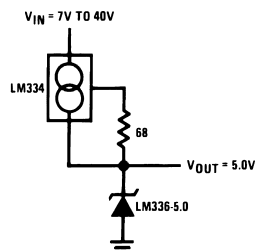
Figure 25. Wide Input Range Reference
