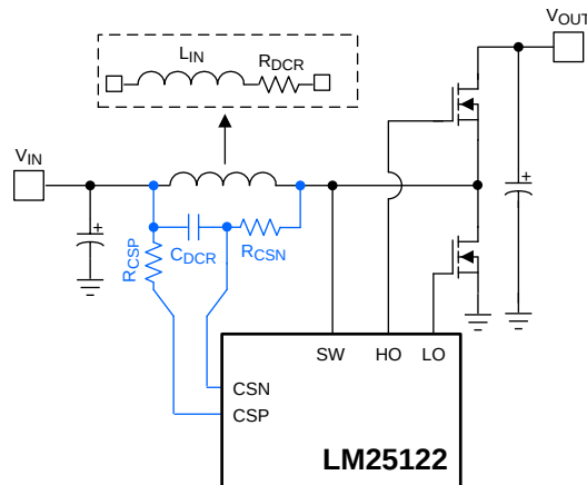
Figure 35. DCR Sensing
