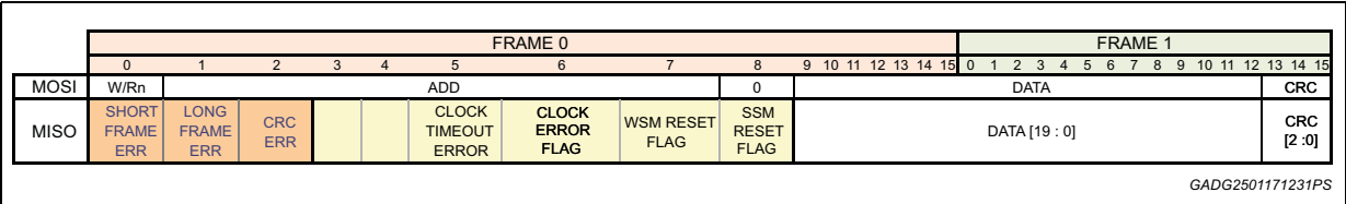
Figure 24. GSW[8..0] bits
