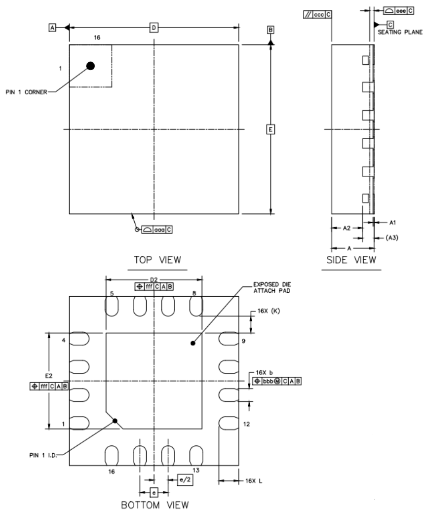
QFNWB3x3-16L-B (P0.50T0.75) 封装外形尺寸
