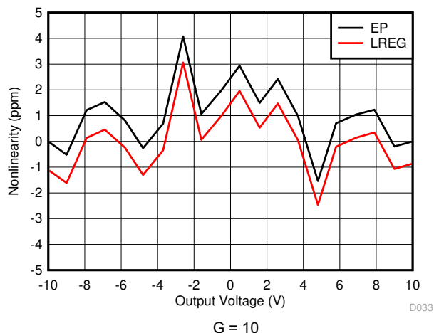
图 7-34. Gain Nonlinearity
