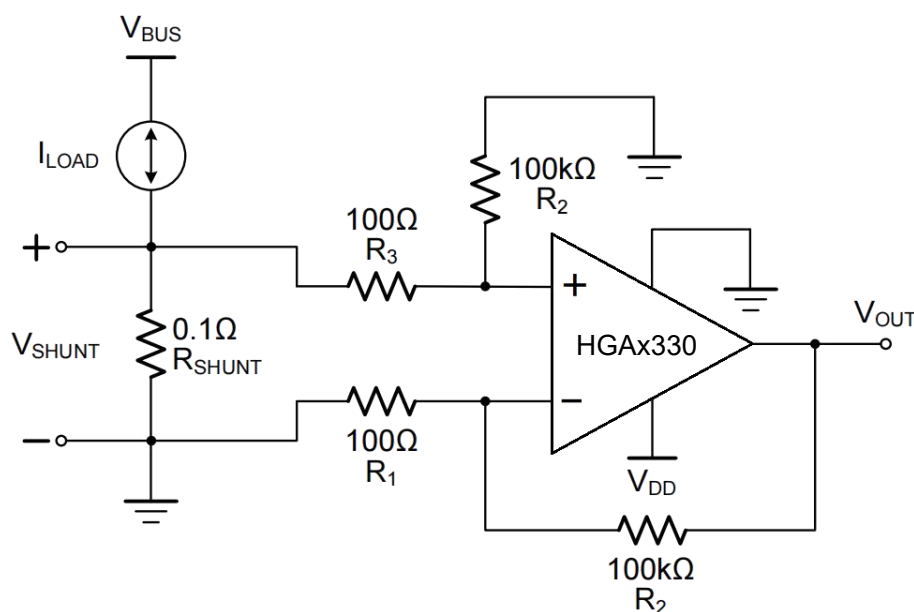
Figure 5. Low-Side Current Sensing Circuit
