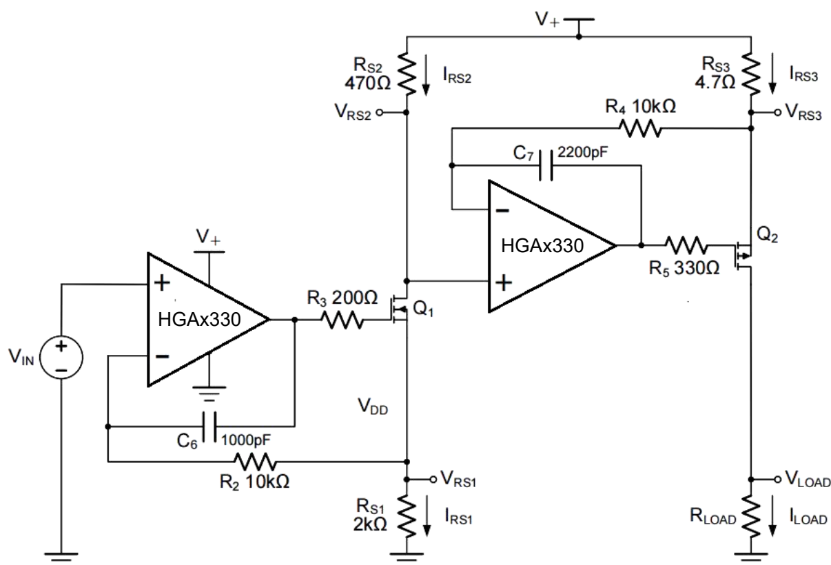
Figure 8. Bidirectional Current-Sensing Schematic
