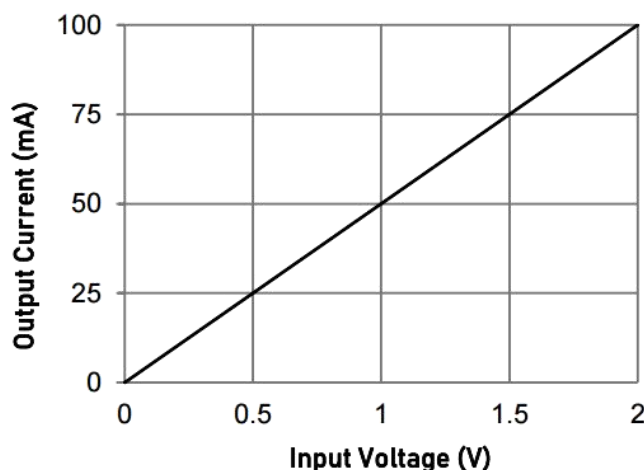
Figure 9. Measured Transfer Function for High-Side V-I Converter
