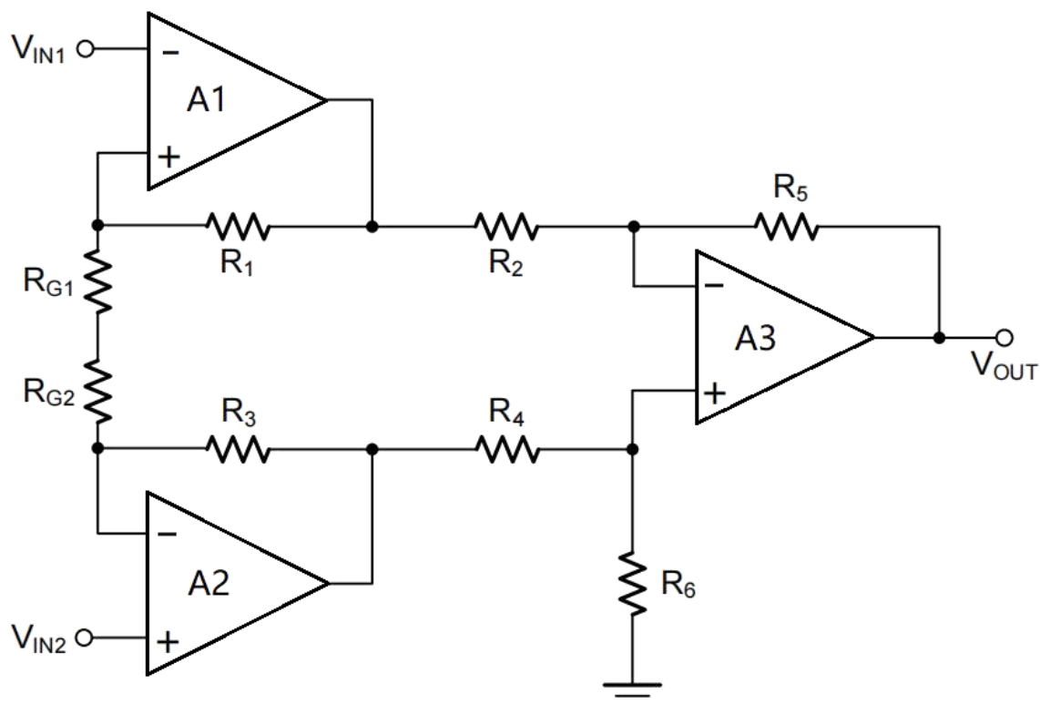
Figure 10. Discrete 3-Op-amp Instrumentation Amplifier
