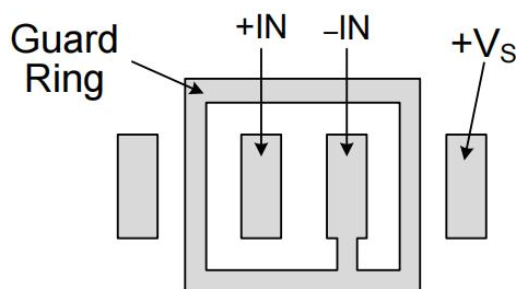
Figure 4. Use a guard ring around sensitive pins
