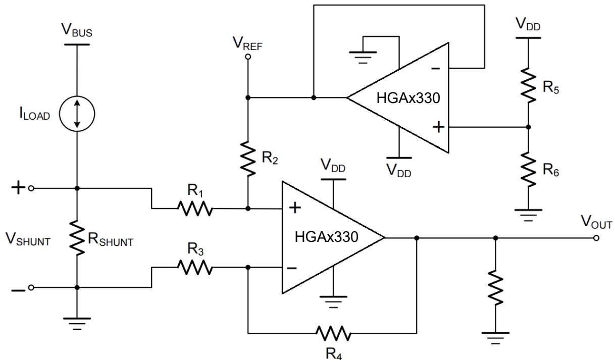
Figure 6. Bidirectional Current-Sensing Schematic
