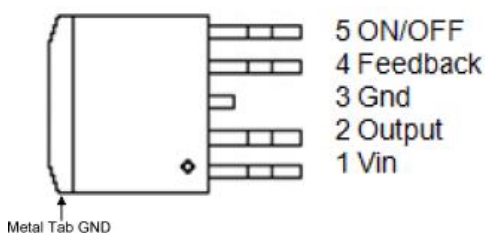
TO -252-4
