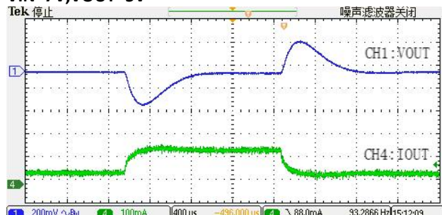
Load Transient (50mA to 150mA) VIN=7V, VOUT=5V
