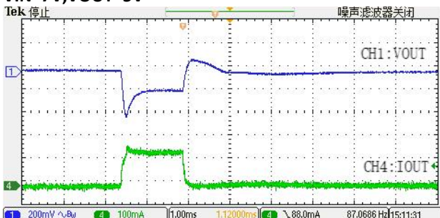
Load Transient (1mA to 150mA) VIN=7V, VOUT=5V
