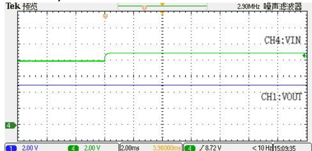
VOUT=5V, Iout=0mA
