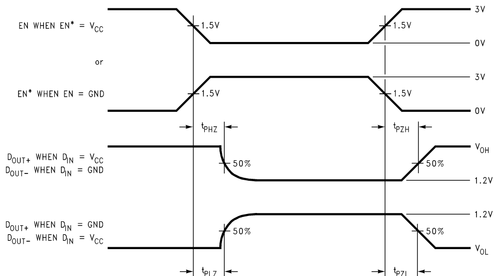
Figure 7. Driver TRI-STATE Delay Waveforms
