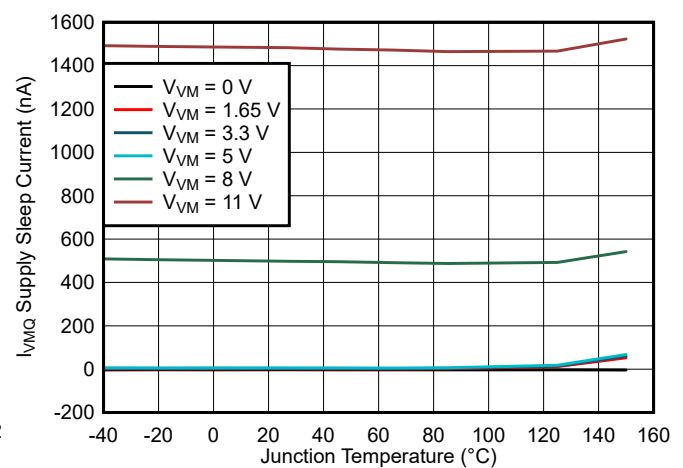
Figure 7-2. Sleep Current ( I_{VMQ} ) vs. Junction Temperature ( T_J )
