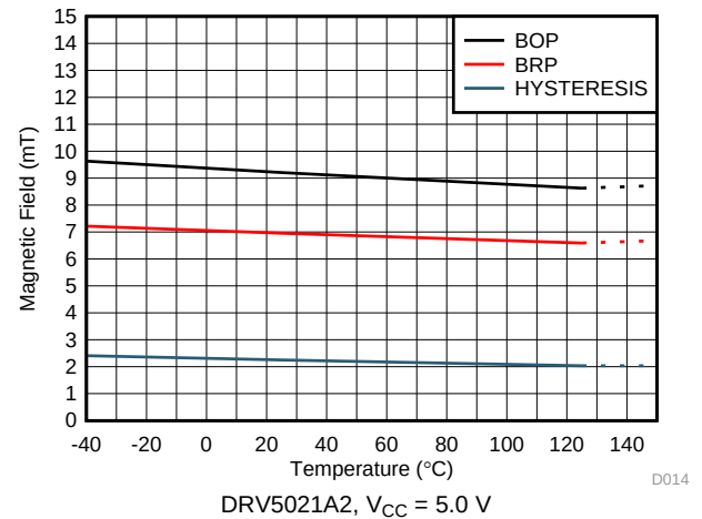
图 4. Magnetic Threshold vs Temperature
