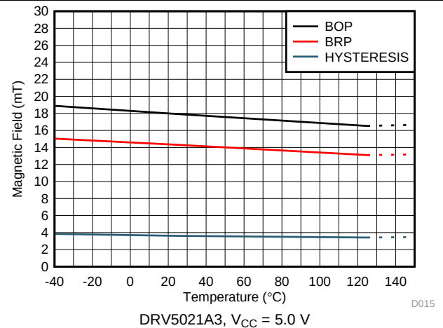
图 6. Magnetic Threshold vs Temperature
